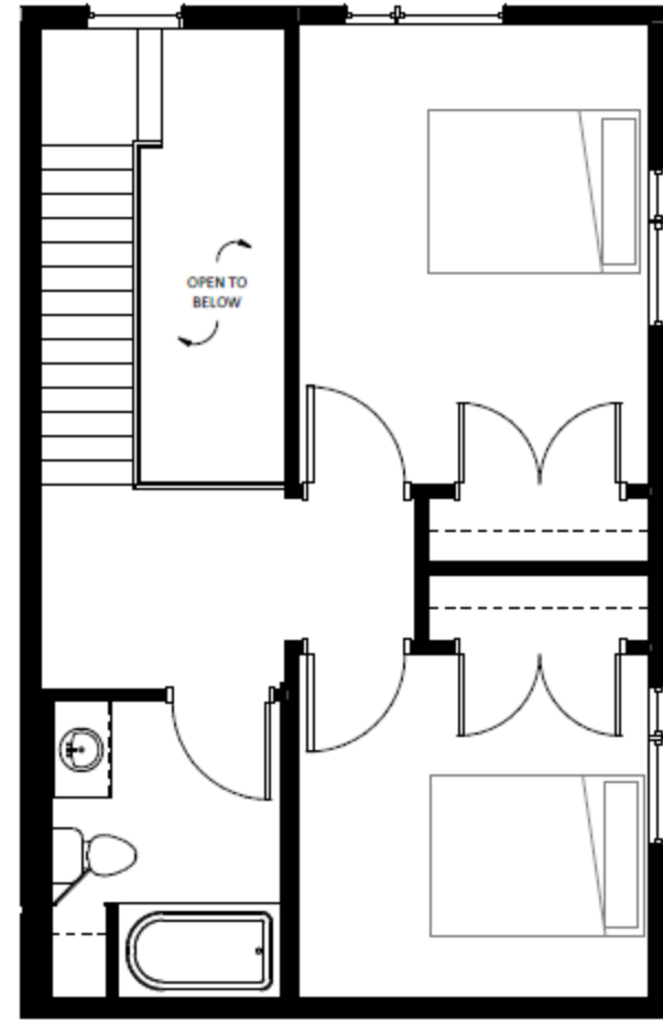
2 2 B.R. LOFT UNIT - 2C UPPER LEVEL SCALE: 1/4" = 1'-0"
