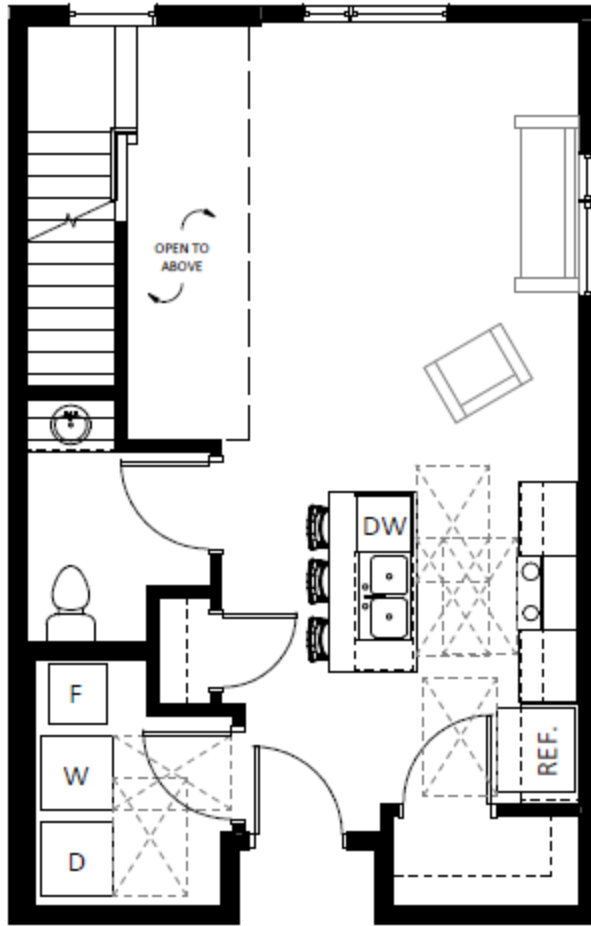
1 2 B.R. LOFT UNIT - 2C LOWER LEVEL - 999 SF SCALE: 1/4" = 1'-0"
