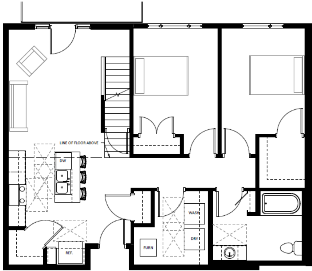
1 2 B.R. W/ DEN LOFT UNIT - 2E LOWER LEVEL - 1,160 SF SCALE: 1/4" = 1'-0"
