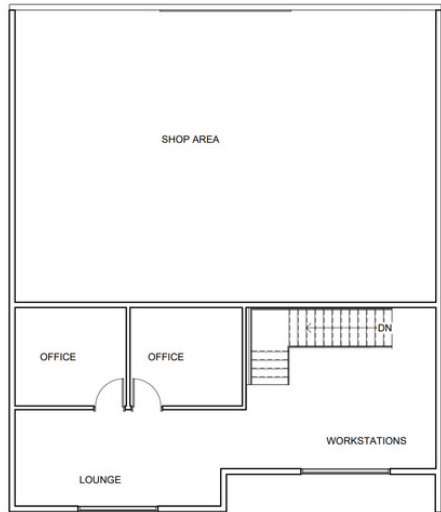
② 46x50 Second Floor W/ Office 1/8" = 1'-0"
