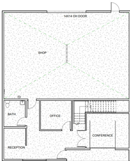
① 46x50 W/ Office 1/8" = 1'-0"
